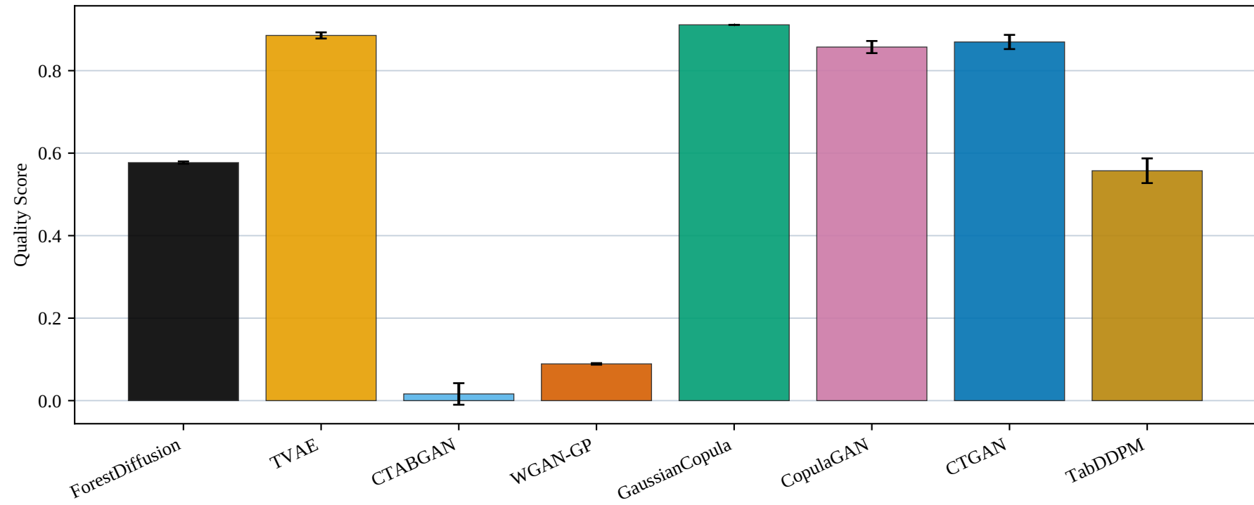
CDC Diabetes — Quality Score (mean \pm SD, 10 seeds)
